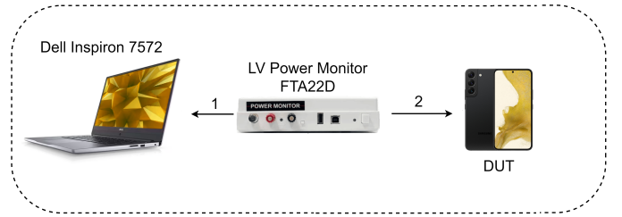
Fig. 2. High-Level Configuration of the Display Power Consumption Measurements Testbed.
