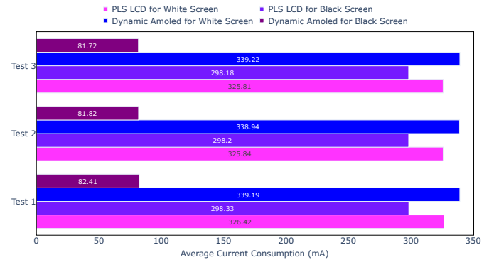
Fig. 6. Test scenarios defined to measure power consumption under White and Black screens.
