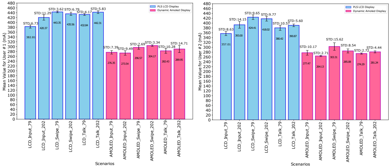
Fig. 16. Average Current Consumption for both users. Left) User 1 and right) User 2.
