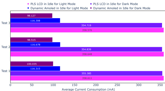
Fig. 5. Test scenarios defined to measure power consumption under Light and Dark Mode screens.
