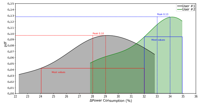
Fig. 15. PDF of the Difference in Current Consumption of PLS LCD with respect to Dynamic AMOLED.
