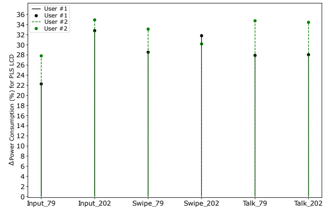
Fig. 14. Percentage Difference in Current Consumption of PLS LCD with respect to Dynamic AMOLED.
