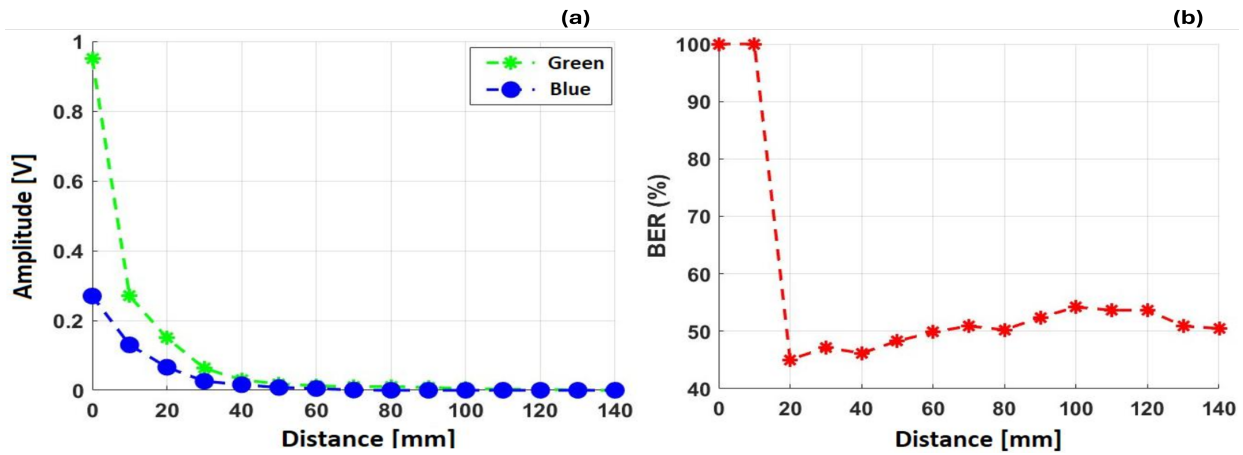
Fig. 12. The results obtained for the voltage generated by the LED and the BER: (a) Energy harvesting in the green and blue channels and (b) Communication in the red channel.
