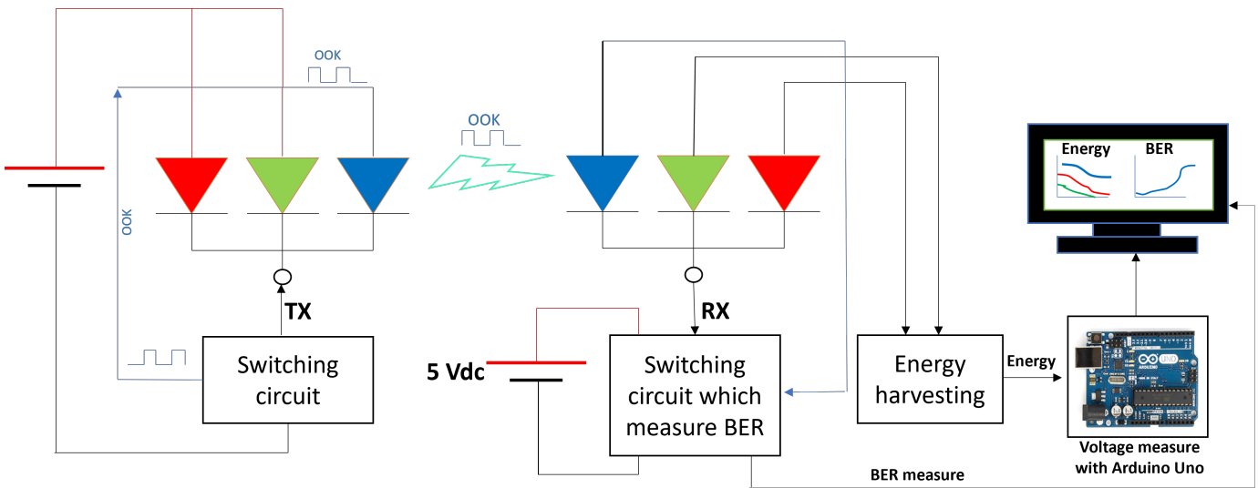
Fig. 5. Experimental setup for BER measurement and voltage accumulation in VLC-ID system.
