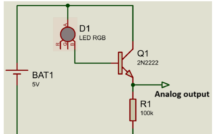
Fig. 11. LED sensor conditioning for VLC-ID communication.
