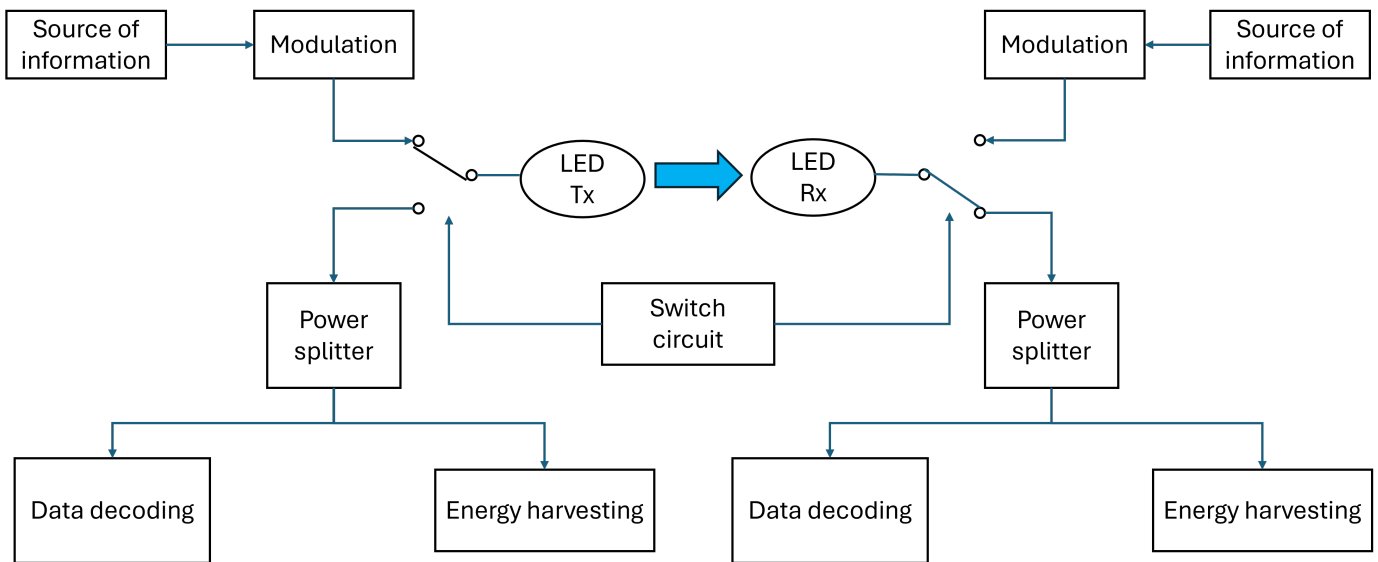
Fig. 3. Conventional power splitting scheme in bidirectional VLC systems.
