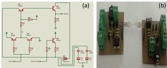
Fig. 1. Bidirectional LED switching circuit for VLC communication and energy harvesting: (a) circuit diagram and (b) experimental prototype.
