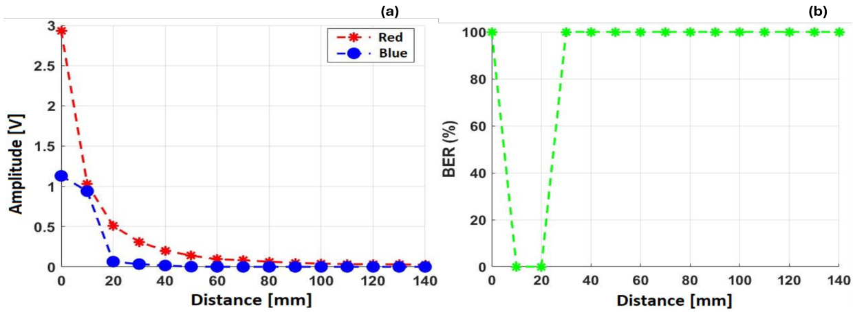
Fig. 13. The results obtained for the voltage generated by the LED and the BER: (a) Energy Harvesting in the red and blue channels and (b) Communication in the green channel.
