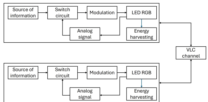
Fig. 4. Simplified power splitting model with RGB LED for simultaneous communication and energy accumulation.
