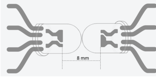
Fig. 9. Distance between LEDs and optical concentration in VLC-ID system.
