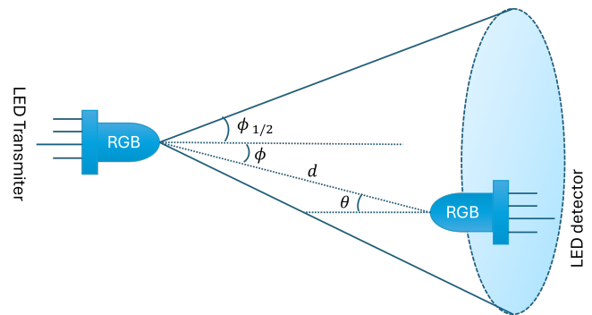
Fig. 7. LED RGB transceiver Model with incidence angle \theta and irradiance angle \phi .
