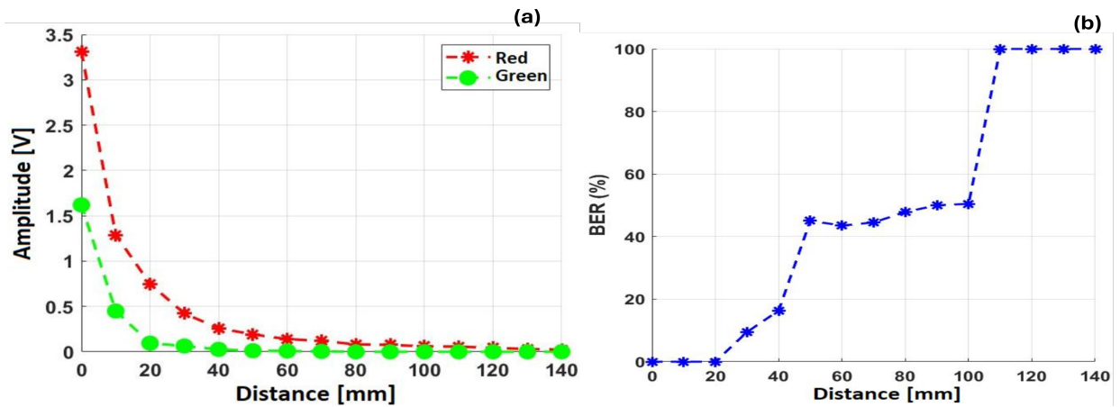
Fig. 14. The results obtained for the voltage generated by the LED and the BER: (a) Energy Harvesting in the green and red channels and (b) Communication in the blue channel.
