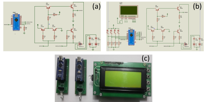
Fig. 2. Design and implementation of the VLC-ID system: (a) key schematic, (b) lock schematic and (c) prototype.
