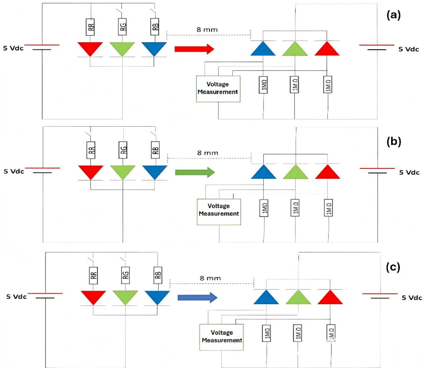
Fig. 10. Conceptual diagram for voltage measurement in energy harvesting and communication channels.
