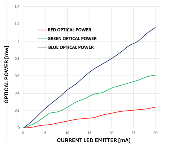
Fig. 8. Current vs. optical power graph for 5mm RGB LED.
