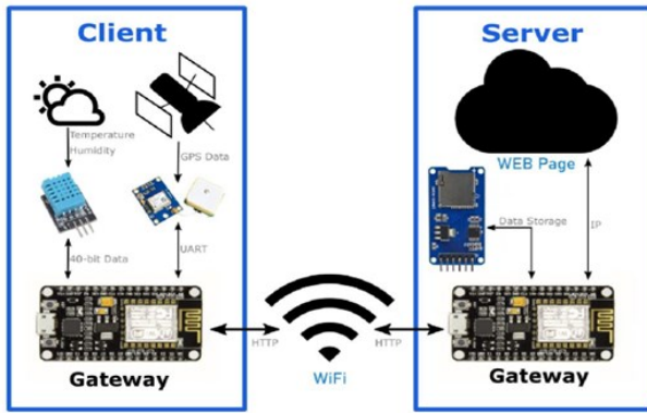
Fig. 1. Communication diagram.
