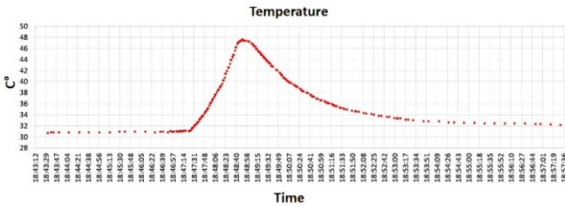
Fig. 12. Temperature from adaptive method.
