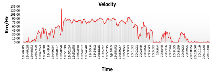
Fig. 9. Velocity plot for route selected points.
