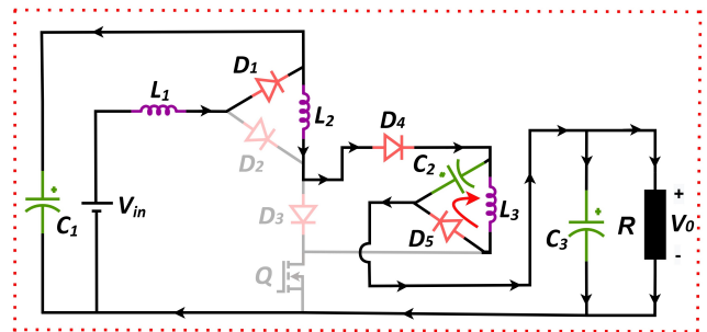
Fig. 4. Mode-II operation.
