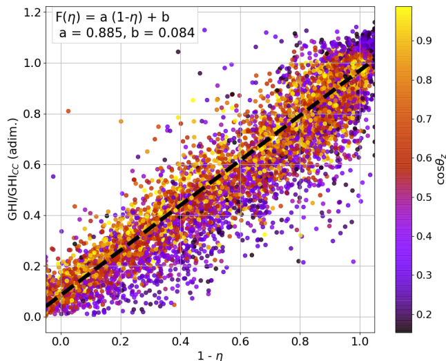
Fig. 2. Example of the linearity between F and (1 - \eta) for hourly data (LE site) [29]. The color of the dots denotes the cosine of the solar zenith angle.
