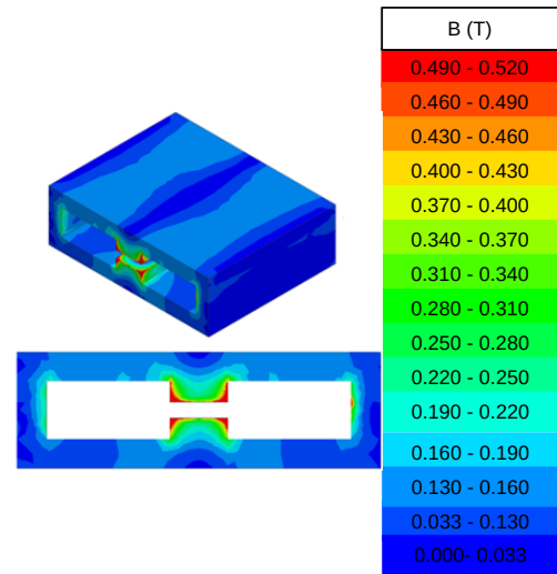
Fig. 15. Magnetostatic Analysis of the Core, Showing Magnetic Flux Densities Below Saturation Levels.
