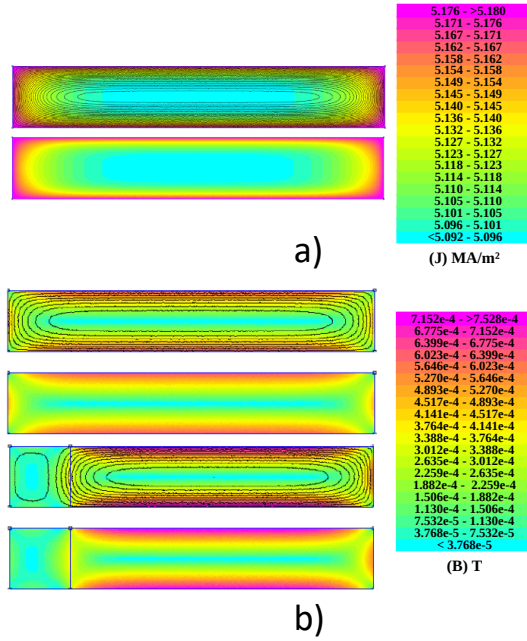
Fig. 17. Current Density Analysis and Induction with Proximity Effect - a) primary skin effect b) primary proximity effect.
