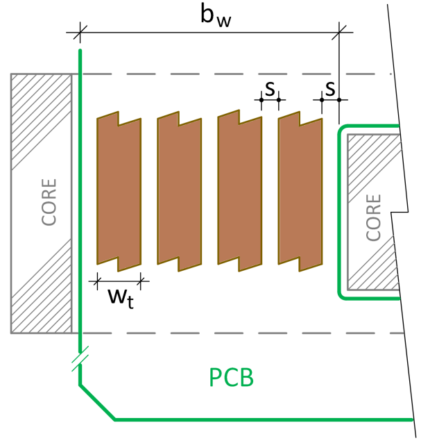
Fig. 8. Layout of the PCB Tracks and the Winding Parameters Used in the Track-Width Calculation.
