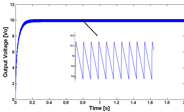
Fig. 23. Measured output voltage of the converter, reaching 10 V with 400 mV pp ripple at steady state.
