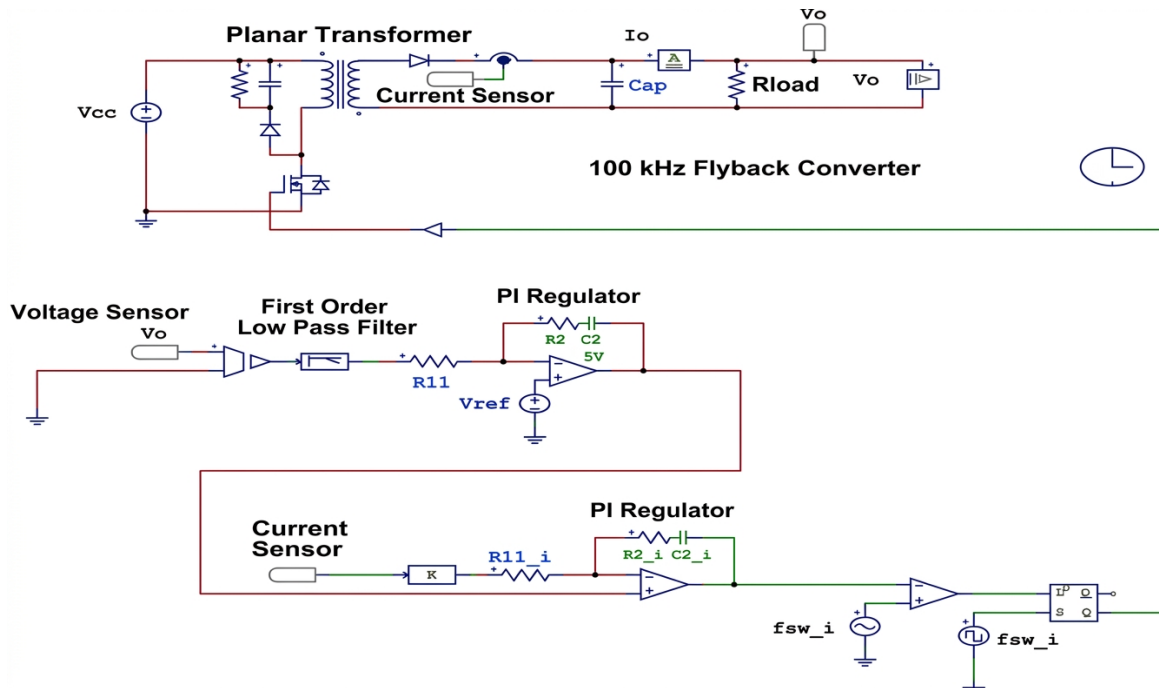
Fig. 22. Schematic of the flyback converter with the designed PTT, including the control loop, implemented in PSIM.
