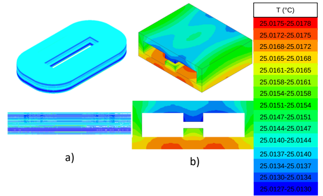
Fig. 16. Core Thermal and Windings Thermal Analysis - a) coil temperature b) core temperature.
