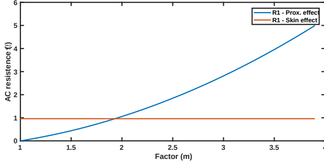
Fig. 9. Estimated AC Resistances in the Primary Side as a Function of the m Factor, Showing Skin and Proximity Effects.
