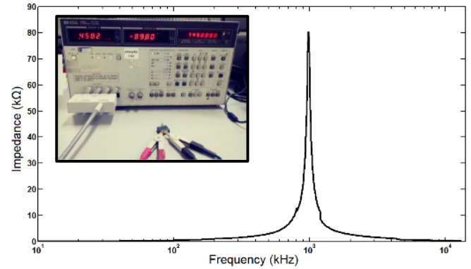
Fig. 19. Measured impedance Z(\omega) at the primary terminals, showing the resonance frequency f_r well separated from the operating frequency.
