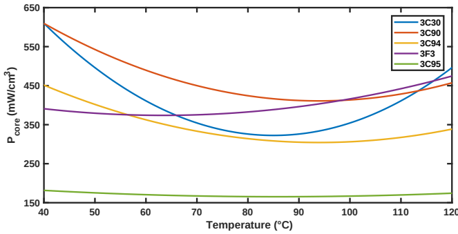
Fig. 6. Power Loss Density at 100kHz and 160mT.
