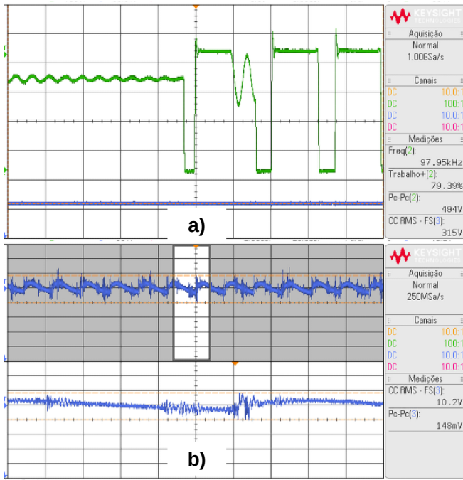
Fig. 21. Measured Voltage and Current Waveforms of the Primary Switch - a) primary switch b) output ripple
