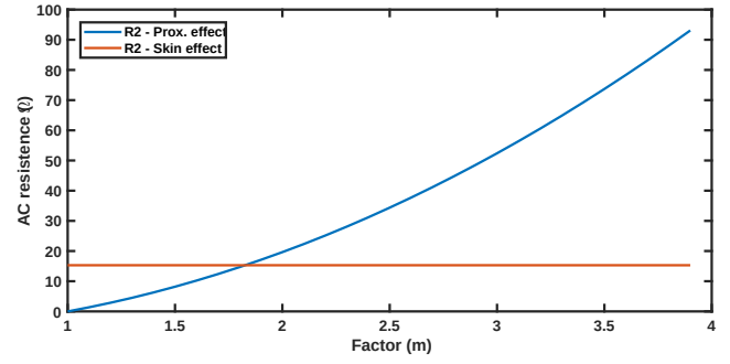
Fig. 10. Estimated AC Resistances in the Secondary Side as a Function of the m Factor, Showing Skin and Proximity Effects.
