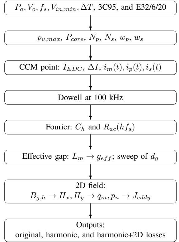
Fig. 11. Flowchart of the code for the 20 W case.
