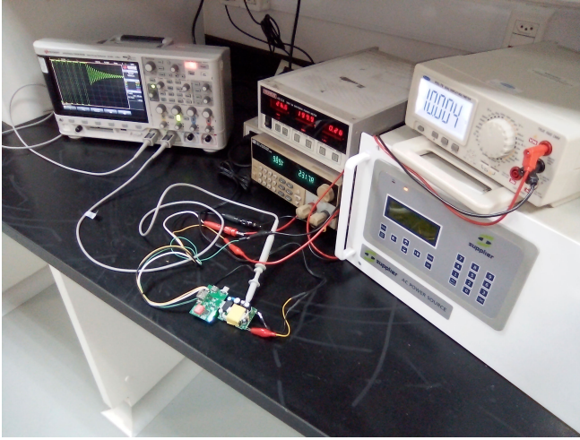
Fig. 20. Experimental Bench Used for the Functional Tests of the Converter With the Designed PTT at V_o = 10 V.
