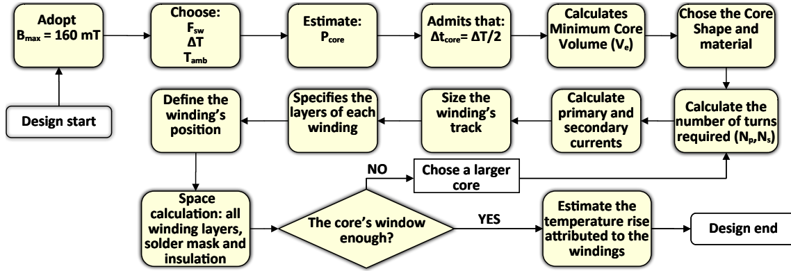
Fig. 5. Type B Methodology: PTT Sizing Procedure Constrained by Temperature Rise and Magnetic Flux Density.
