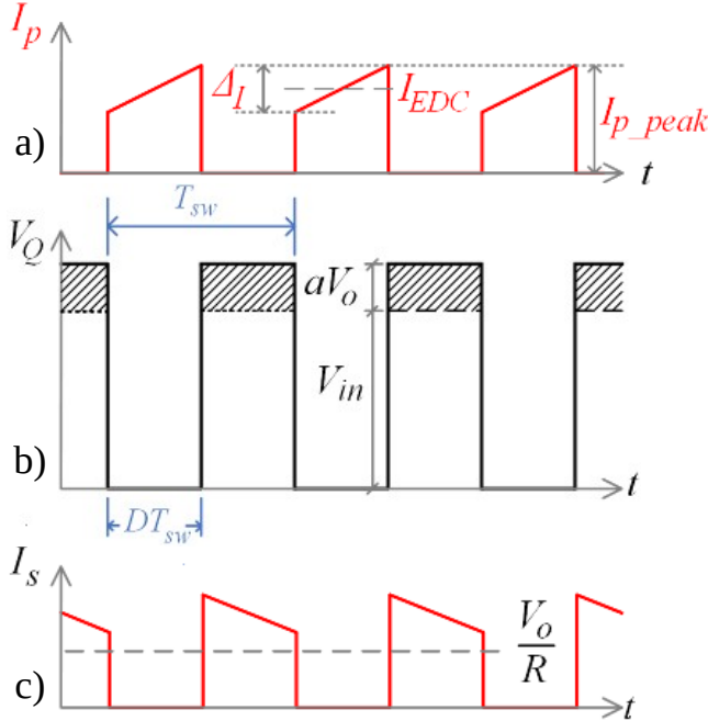
Fig. 4. Current and Voltage Waveforms of Switch Q Operating in CCM - a) primary current b) switch voltage c) secondary current. Adapted [42]
