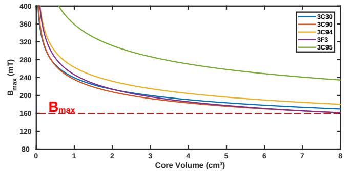
Fig. 7. Maximum Flux Density at 100kHz and 100°C.
