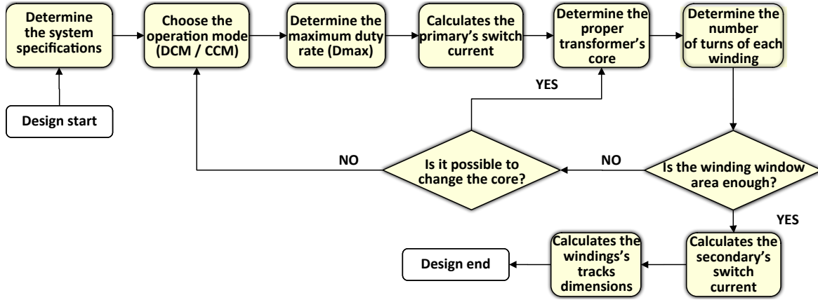
Fig. 3. Type A Methodology: PTT Sizing Steps for Single Secondary Winding Applications.
