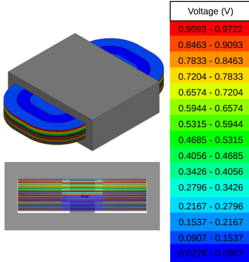
Fig. 14. Electrostatic Analysis of the Winding Tracks, Showing Sufficient Insulation Between Adjacent Turns.
