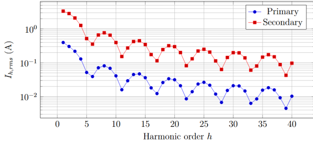
Fig. 12. Spectrum of the CCM Currents Reconstructed from the Operating Point of Methodology B.
